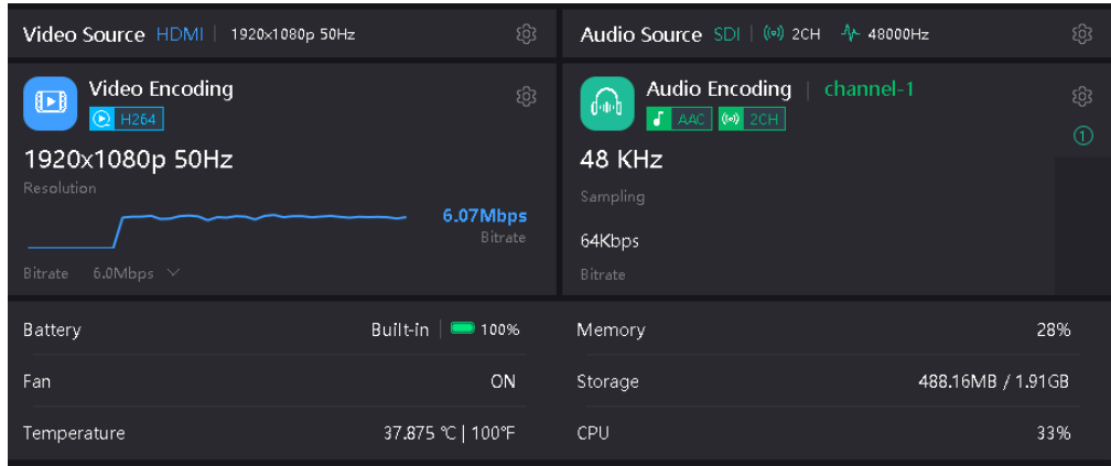
Figure 26: Web Management Backend Homepage Dashboard
